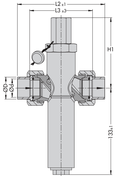
Connecting parts with flat gasket
