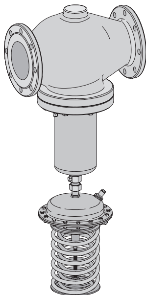
Type 2422/2424 Pressure Reducing Valve
