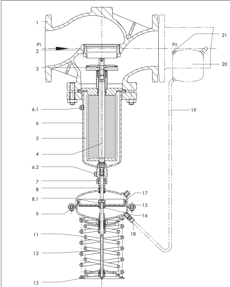
Fig. 1 · Design and principle of operation
