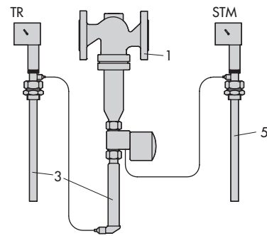
Fig. 8 · Temperature Regulator and Safety Temperature Monitor (TR/STM) with Type 2231 Control Thermostat and Type 2213 Safety Thermostat, Type 2114/2231/2213
