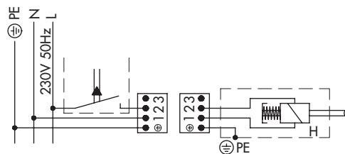
Fig. 13 · Circuit diagram of the electromagnetic release device
