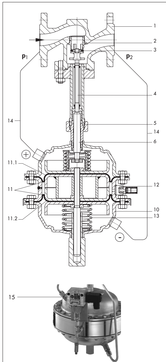
Fig. 3 · Functional diagram
