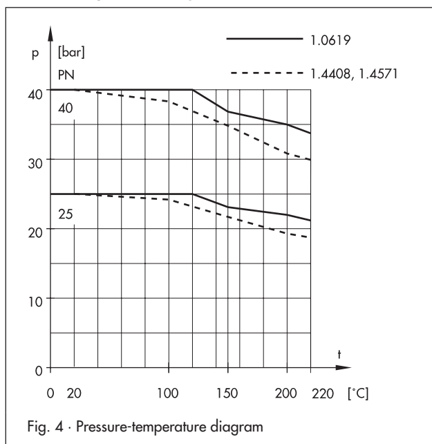
Pressure-temperature diagram – acc. to DIN EN 12516-1 –
