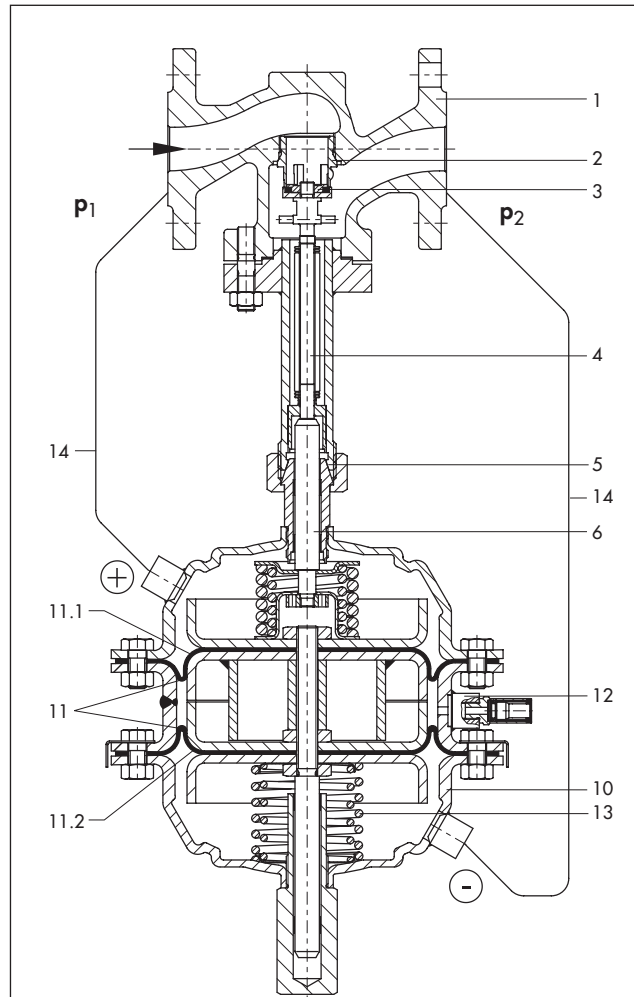
Fig. 3 - Functional diagram
