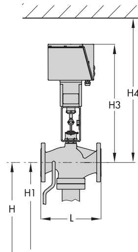
Type 42-36 E with Type 3274/3374 Actuator
