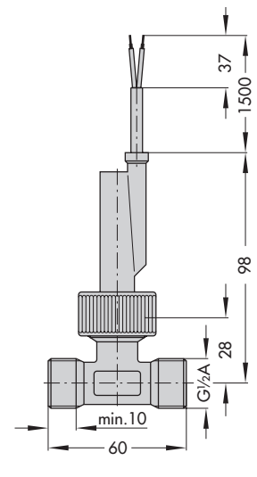
Circulation circuit connection (incl. gasket) (order no. 1400-9232)
