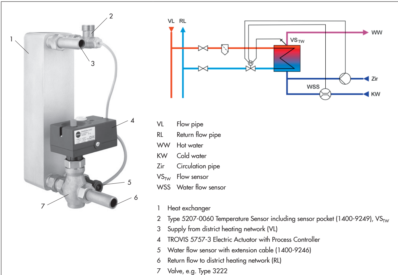
Fig. 5: Sample application: TROVIS 5757-3 with Type 5207-0060 Pt 1000 Sensor including sensor pocket and water flow sensor
