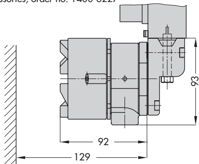
Fig. 8: Dimensions
