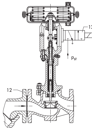
Fig. 3: Type 3241-1-Oil with bellows seal and plug with high-performance metal sealing
