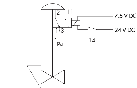
Fig. 4: Functional diagram showing version without positioner
