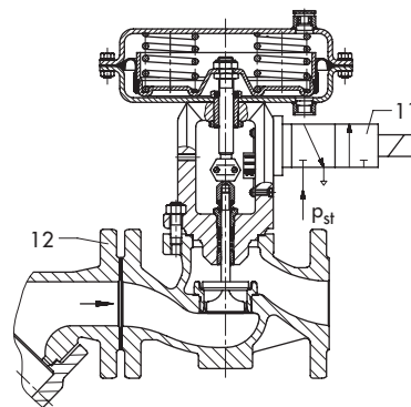
Fig. 2: Type 3241-1-Oil Standard version with soft-seated plug
