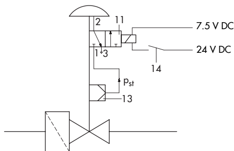
Fig. 5: Functional diagram showing version with positioner
