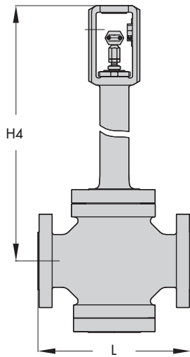
Type 3254 with bellows seal or extension bonnet
