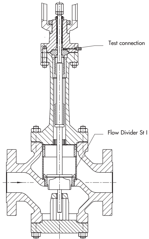
Fig. 4 · Type 3254 Globe Valve with Flow Divider St I and additional bellows seal with test connection
