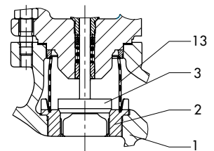
Fig. 1 · Flow Divider St I, installed in Type 3241 Valve
