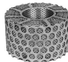
Fig. 3 · Flow Divider St III, installed in Type 3254 Valve
