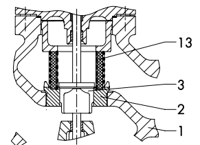
Fig. 3 · Flow Divider St III, installed in Type 3254 Valve
