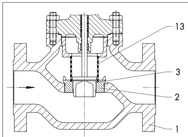
Fig. 5: Type 3251 Valve with flow divider St I
