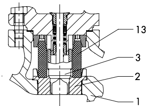
Fig. 2 · Flow Divider St III, installed in Type 3241 Valve
