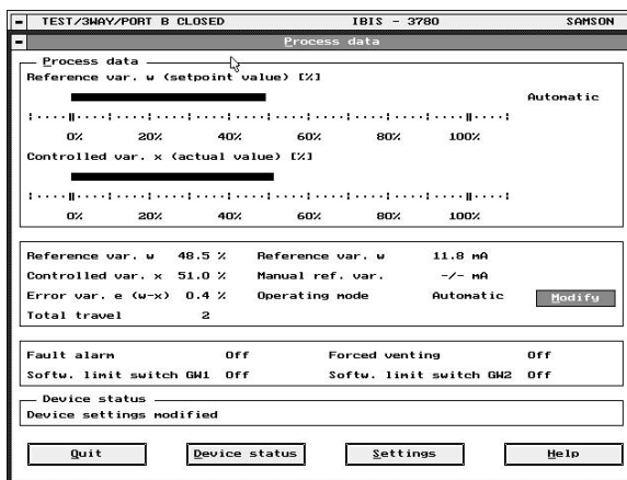
Fig. 4 · Display of the process values by means of the program package IBIS (Intelligent Operating and Information System)
