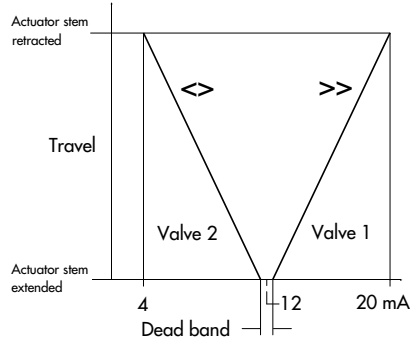
Fig. 12 · Split-range operation (two valves operating in opposite directions)
