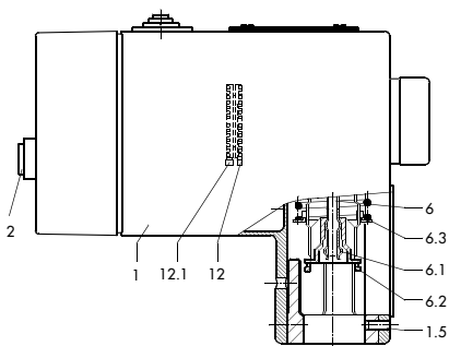
Fig. 4 · Type 5822-10, -20, -30, -40 operating direction OUT (Type 5822-11, -21, -31, -41 operating direction IN) form-fit connection
