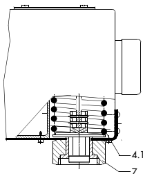
Fig. 5 · Type 5822-50, -60, -70 force-locking connection
