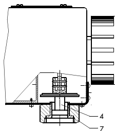
Fig. 3 · Type 5821-5, -6 force-locking connection
