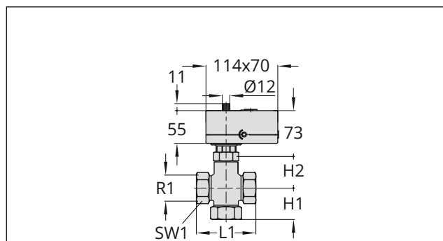
Fig. 9: Type 3226/5857 Electric Control Valve: DN 15 to 25 Type 3226/5757-7: DN 15 to 25
