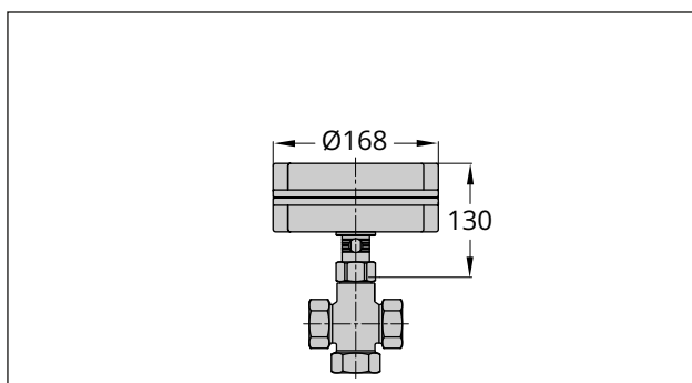
Fig. 12: Type 3226/2780-1 Pneumatic Control Valve: DN 15 to 50
