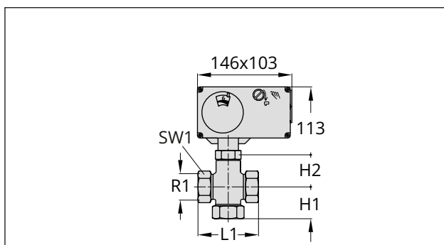
Fig. 10: Type 3226/5724-8 Electric Control Valve: DN 15 to 50 Type 3226/5725-8: DN 15 to 50
