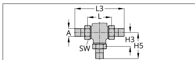
Fig. 6: Type 3226 Three-way Valve with male thread connections and threaded ends
