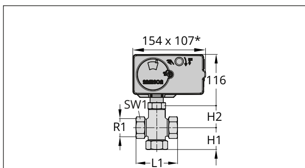
Fig. 11: Type 3226/5827 Electric Control Valve: DN 15 to 50
