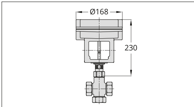
Fig. 13: Type 3226/2780-2 Pneumatic Control Valve: DN 15 to 50
