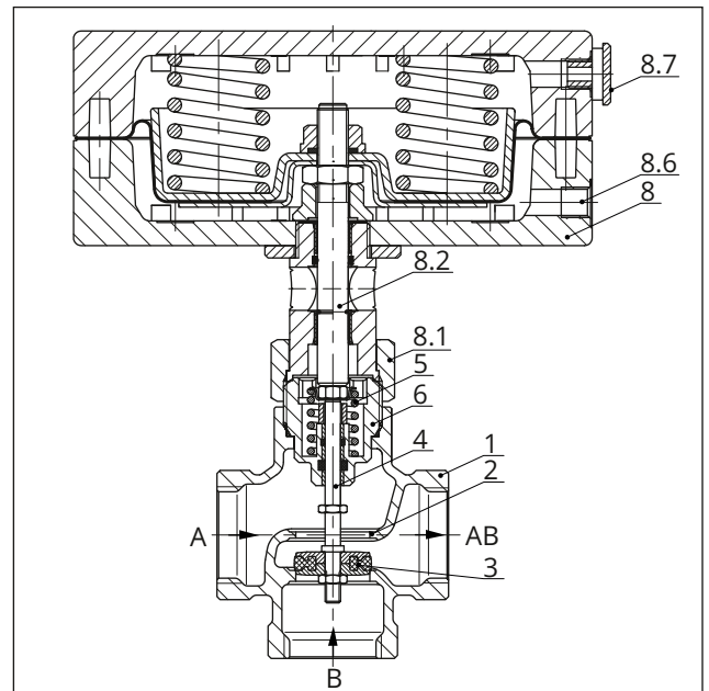
Fig. 4: Type 3226/2780-1 Pneumatic Control Valve (mixing valve)
