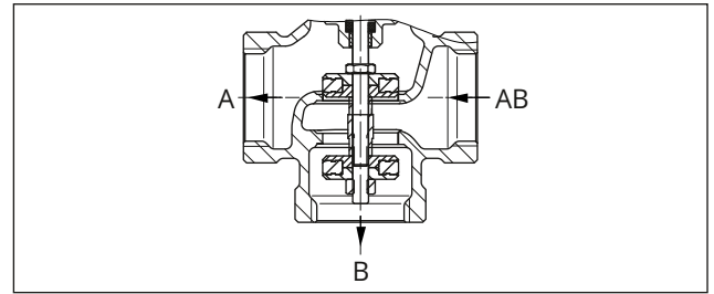
Fig. 3: Type 3226 (diverting valve)
