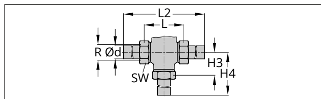
Fig. 5: Type 3226 Three-way Valve with male thread connections and welding ends
