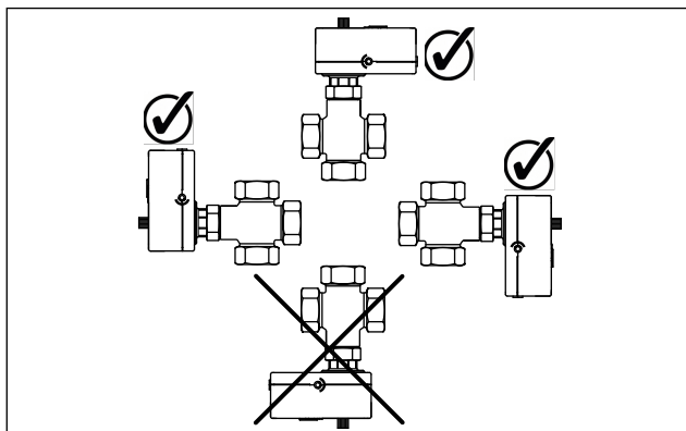
Fig. 14: Mounting position
