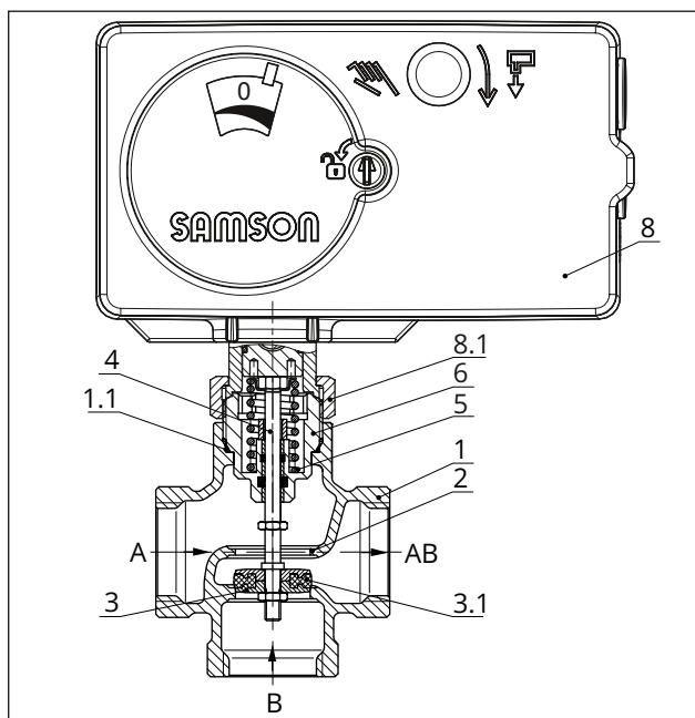
Fig. 2: Type 3226/5827 Electric Control Valve (mixing valve)
