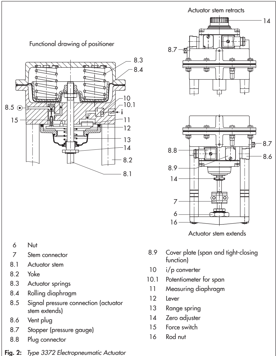
Fig. 2: Type 3372 Electropneumatic Actuator
