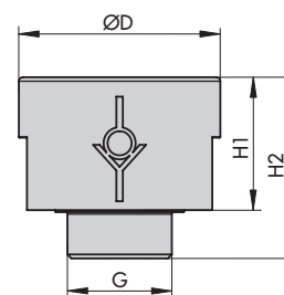
Fig. 5a: Check valve (1790-7408 and 1790-9645)
