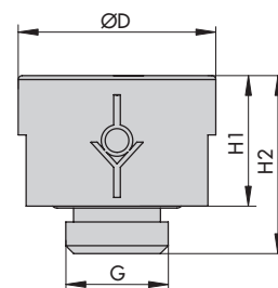
Fig. 5b: Check valve (1790-7253 and 1790-9646)
