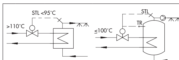
Fig. 1: DHW heating according to DIN 4753
