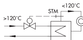
Fig. 2: Heating system with safety temperature monitor according to DIN 4747-1
