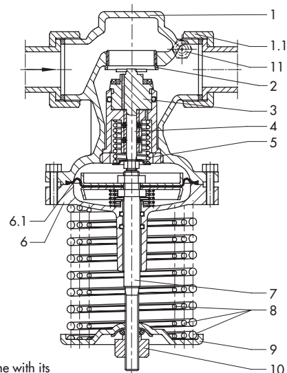
Type 44-2 Pressure Reducing Valve, body with welding ends
