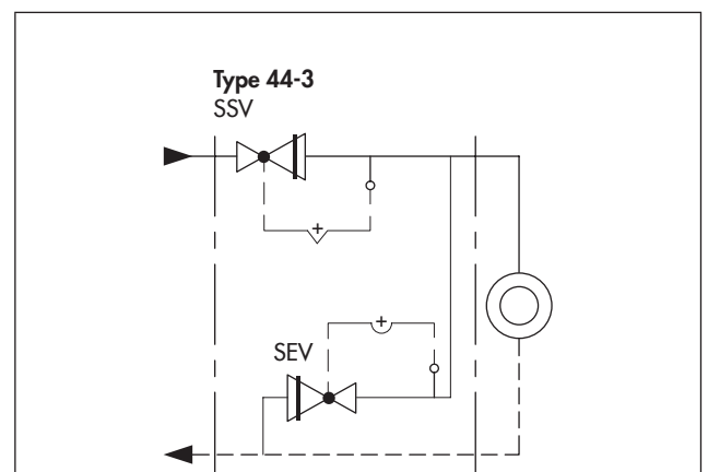
Fig. 1: Protection of a house substation with a Type 44-3 SSV and SEV
