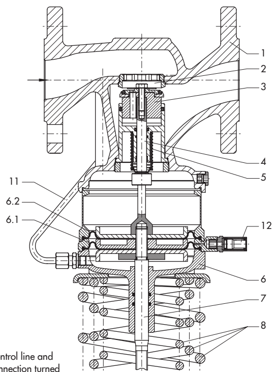
Type 44-3 Safety Shut-off Valve (SSV), flanged valve body
