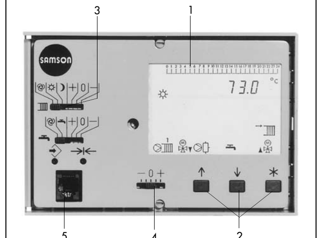
Fig. 2 · Operator controls
