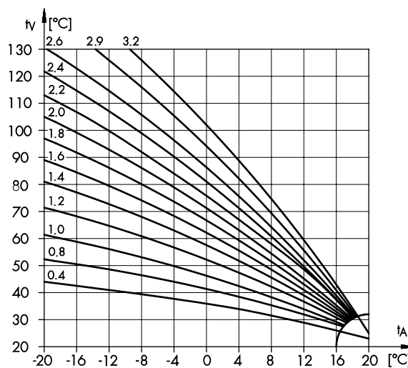
Fig. 4 · Family of heating characteristics
