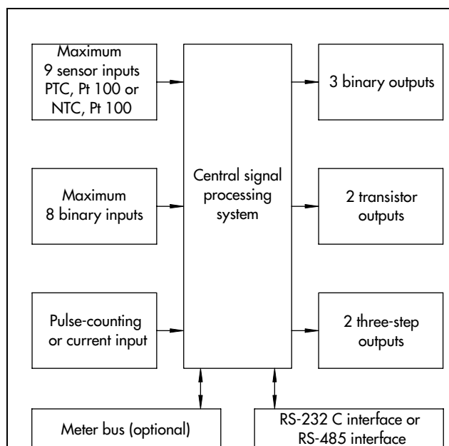
Fig. 3 · Hardware design
