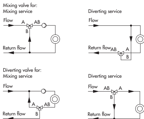
Fig. 4: Typical installations
