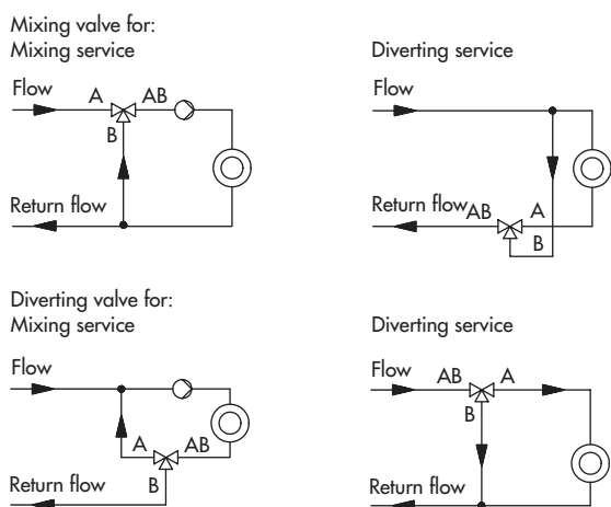
Fig. 4: Typical installations
