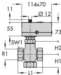
Type 3226/5857: DN 15 to 25 Type 3226/5757-7: DN 15 to 25
