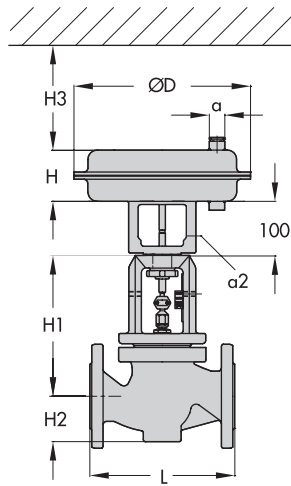
Type 3241-7 with Type 3277 Actuator
