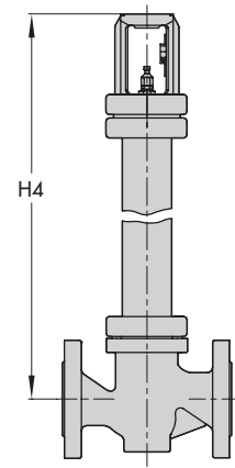
Type 3241 with insulating section
