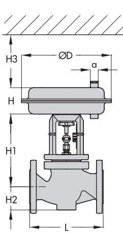
Type 3241-1 with Type 3271 Actuator
