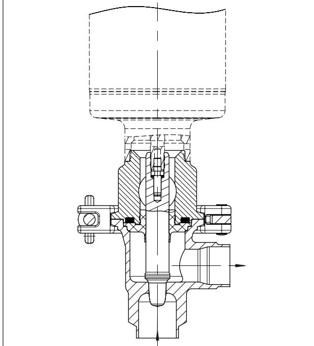
Fig. 4: Type 3347/3379 Control Valve with welding ends Version with cast body
