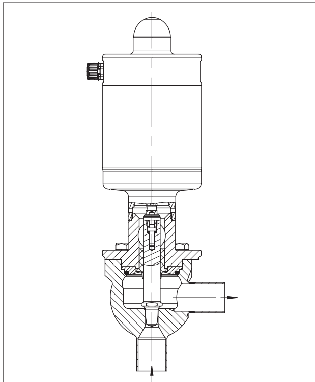
Fig. 3: Type 3347/3379 Control Valve with welding ends Version with bar stock body with bolted bonnet
