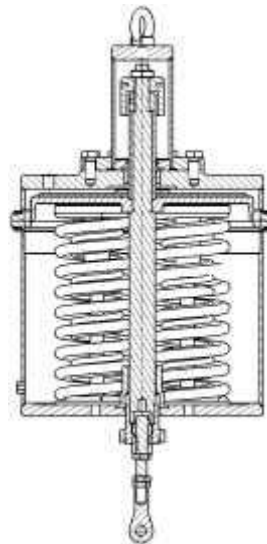
Fig. 2: Sectional drawing of Type MD Actuator
