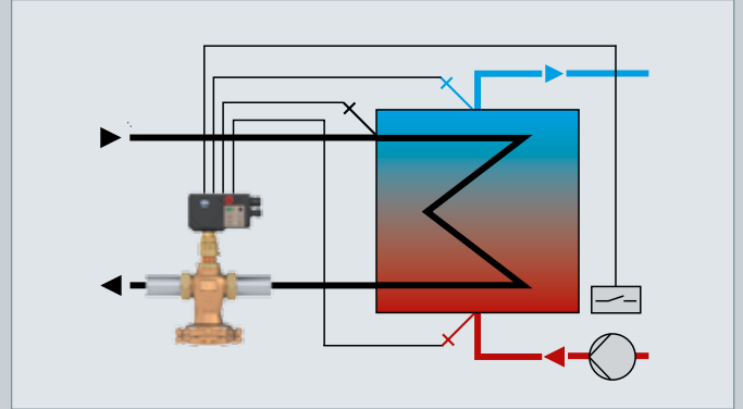
Control of the flow temperature in the secondary circuit taking into account the network supply temperature and the return flow temperature in the secondary circuit
